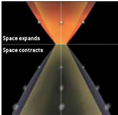
Two nearly empty branes pull each other together. Each is contracting in a direction perpendicular to its motion.
